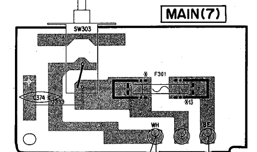
To POWER TRANSFORMER (A) (G, B)
